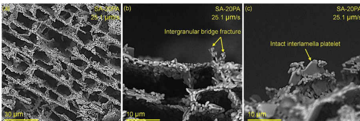
Figure 14: SEM micrographs of a partially deformed ( \sim 10\% engineering strain) SA-20PA scaffold that was processed in the high FFV regime. (a) Loading surface of the specimen revealing limited separation of the lamellae walls. (b) Intergranular fracture of a lamellar bridge without an interlamella platelet. (c) Intact interlamella platelet on the deformed scaffold surface.
