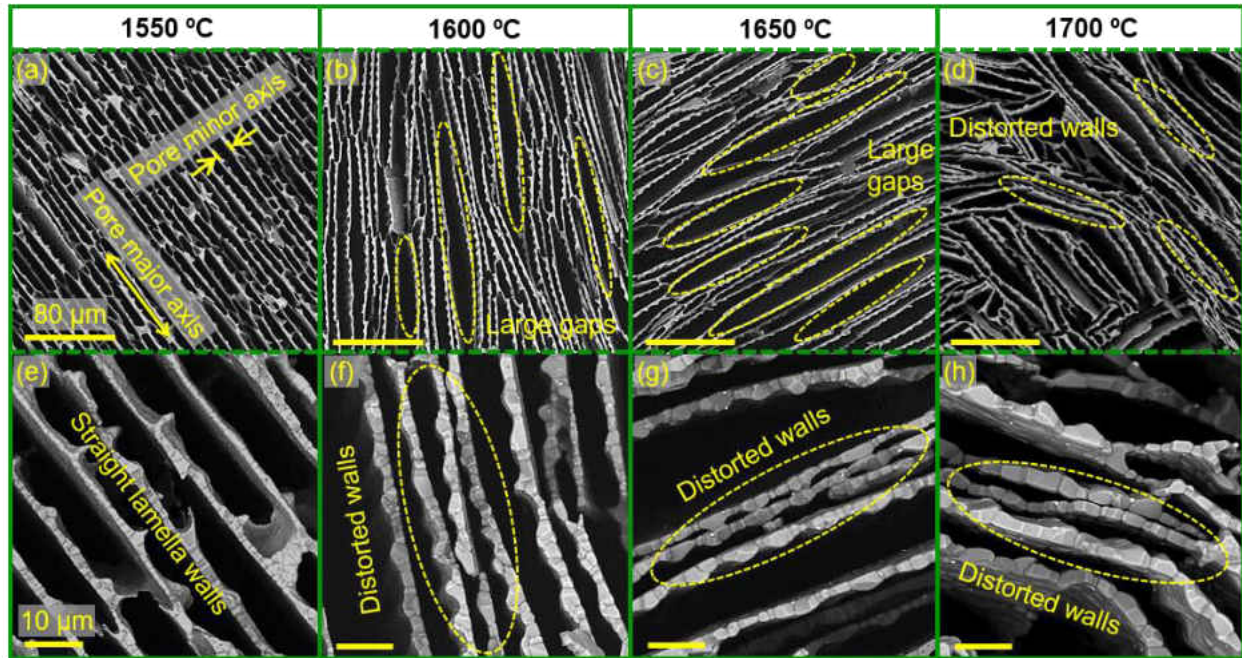
Figure 10: Relatively low- and high-magnification SEM images of the cross-section regions (perpendicular to the ice-growth direction) of the UA-15 materials revealing distortion (bending) of lamella walls with the increasing sintering temperature in the range of 1550–1700 °C. Images in each column belong to the same sintering temperature but captured at two different magnifications.
