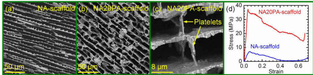
Figure 1: SEM micrographs reveal (a) lamellar pore morphology of the NA-scaffold and (b) dendritic pore morphology of the NA20PA-scaffold, and (c) high magnification SEM micrograph shows lamellar bridge formation through the platelets (ice-growth direction is out of the page). (d) Comparison of uniaxial compressive response of the NA-scaffold and the NA20PA-scaffold.
