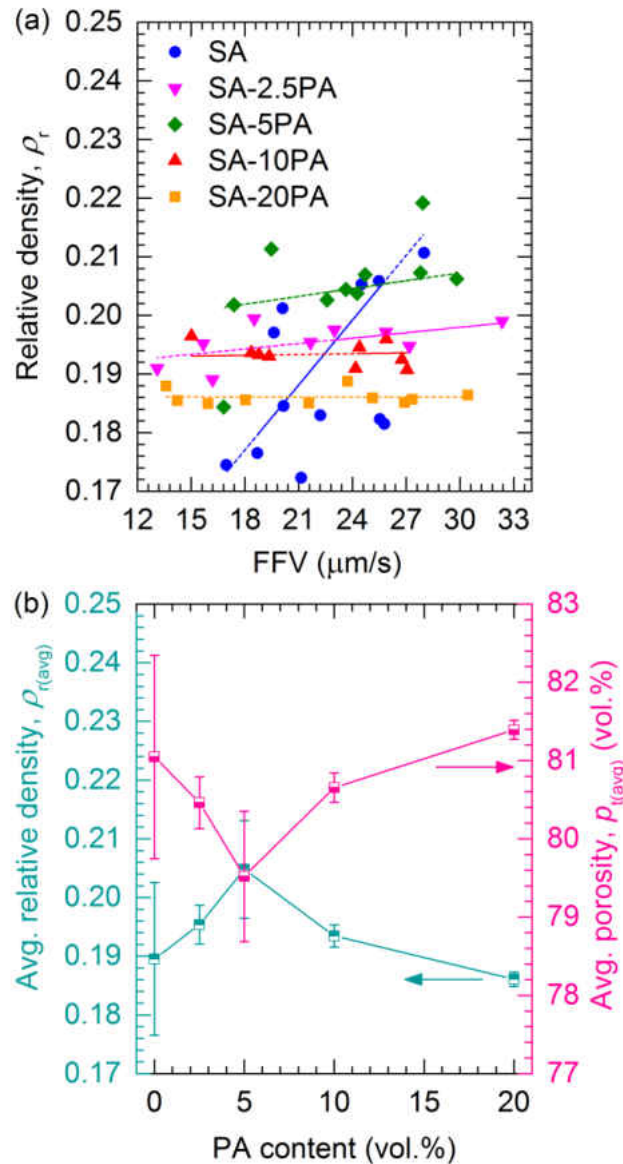
Figure 4: Variation of (a) relative density ( \rho_r ) with FFV and (b) average relative density ( \rho_{r(\text{avg})} ) and average total porosity ( p_{t(\text{avg})} ) with platelets (PA) content.
