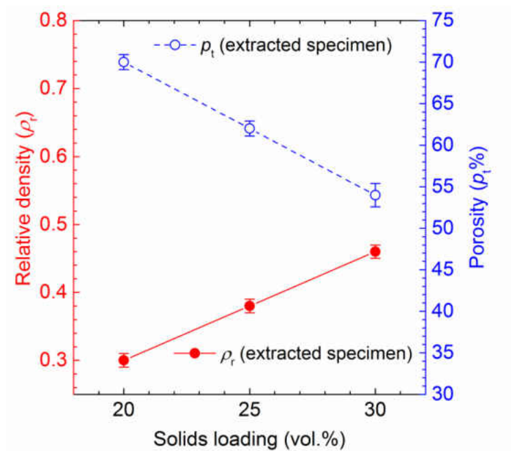
Figure 2: Variation of average relative density ( \rho_r ) and average total porosity ( p_t ) of the extracted specimens from the sintered scaffolds as a function of solids loadings of suspensions.
