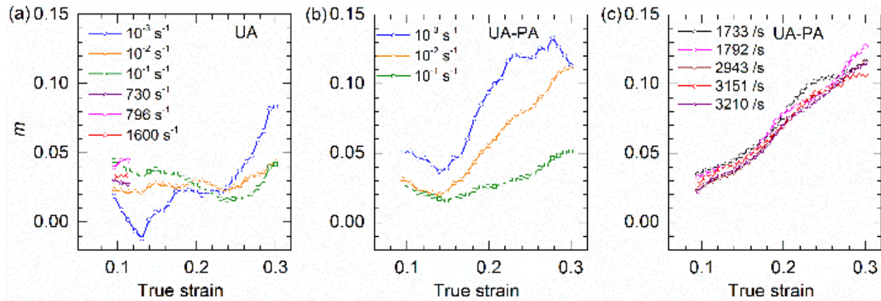
Figure 4: Variation in strain rate sensitivity parameter ( m ) with true strain for (a) UA material in both strain rate regimes, (b) UA-PA material in quasistatic strain rate regime, and (c) UA-PA material in dynamic strain rate regime.
